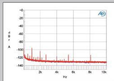
Fig.6 Advance Paris X-CD9, spectrum with noise and spurs of dithered 1kHz tone at -90dBFS with 16-bit data (left channel blue, right red) (20dB/vertical div.).
