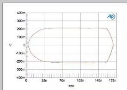
Fig.1 Advance Paris X-CD9, eye pattern of coaxial S/PDIF output carrying 16-bit, 44.1kHz J-Test data (±400mV vertical scale, 175ns horizontal scale).
